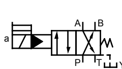
Reverse Mtg. of Solenoid ("L")
