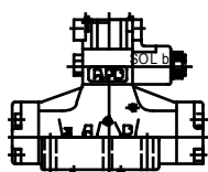
Standard Mtg. of Solenoid
